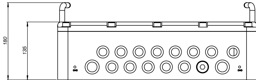
L0QX01 IEC Flameproof Display Enclosure Exid
