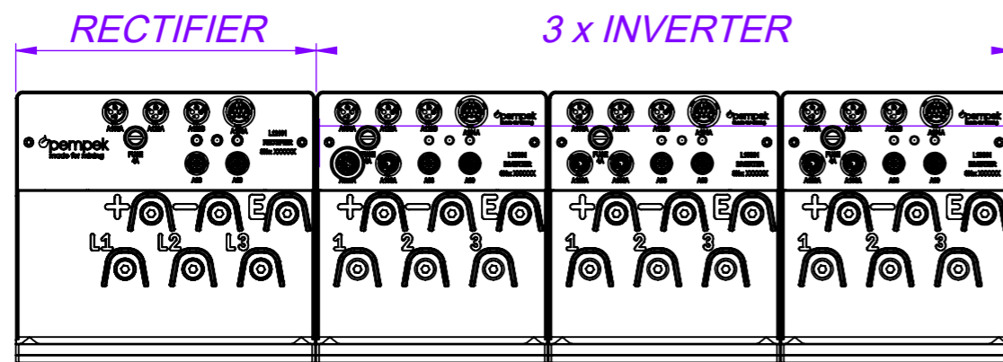
FRONT TERMINALS - M8
