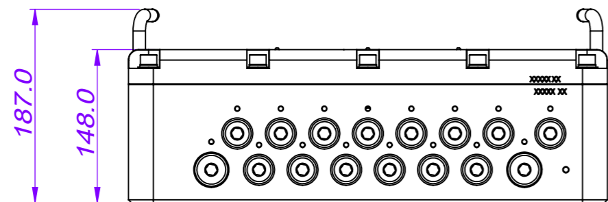
26 x M20 ENTRIES 4 x M25 ENTRIES
